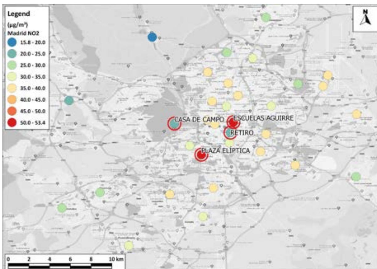
Figure 3-1: 2019 Annual Mean Concentrations NO 2 at Fixed Monitoring Sites in Madrid
