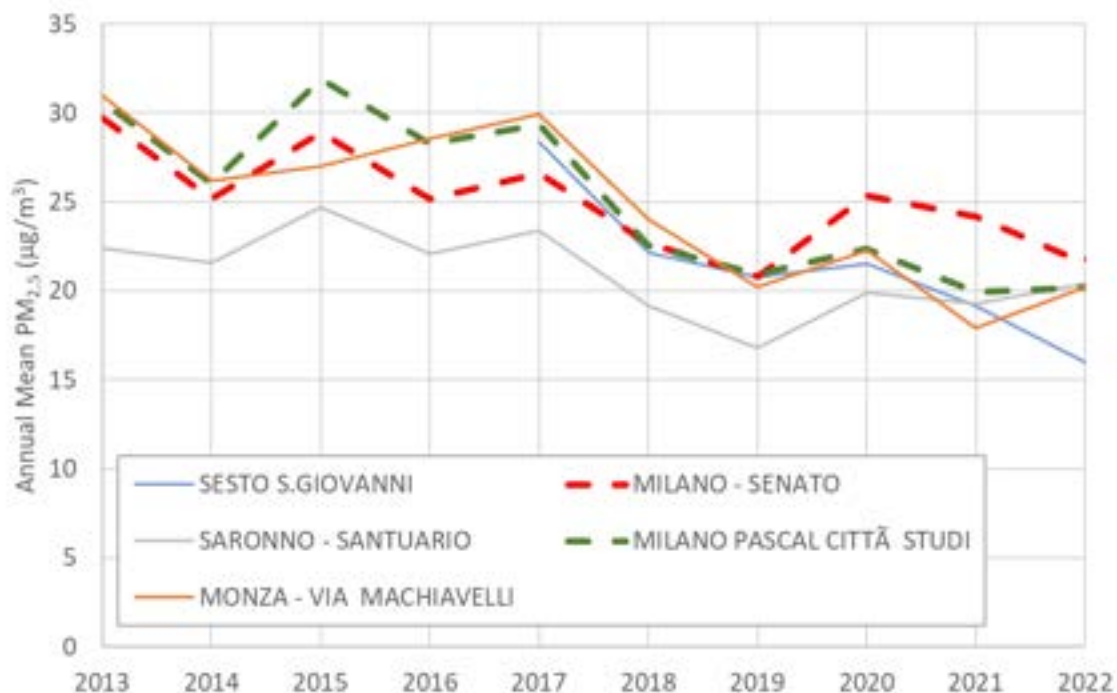
Figure 3-19: Annual Mean PM 2.5 Concentrations at Fixed Monitoring Sites in Milan, 2013 to 2022
