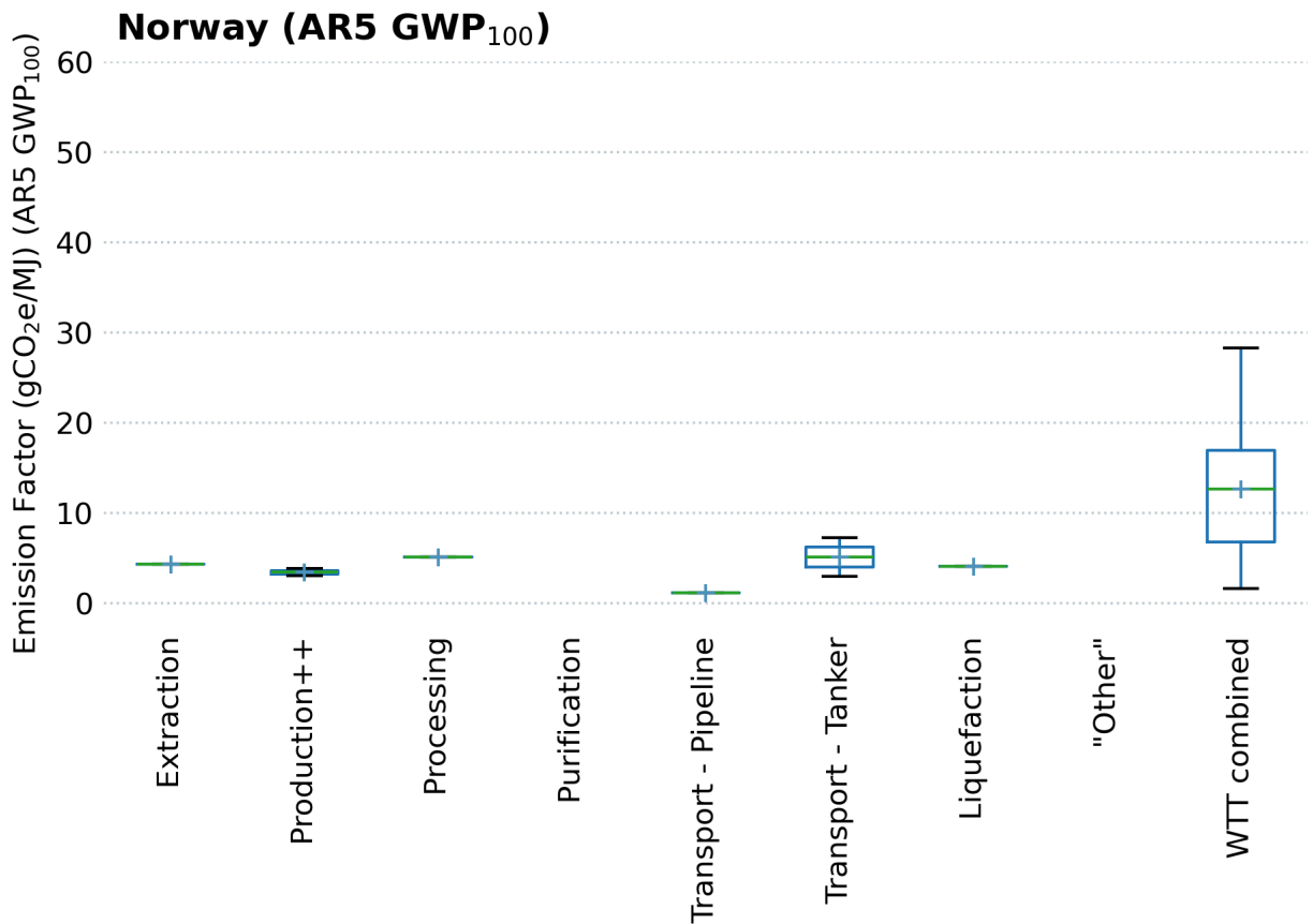
Emission Factors Across LNG Supply Chain in Norway (AR5, GWP 100 , gCO 2 e/MJ)
