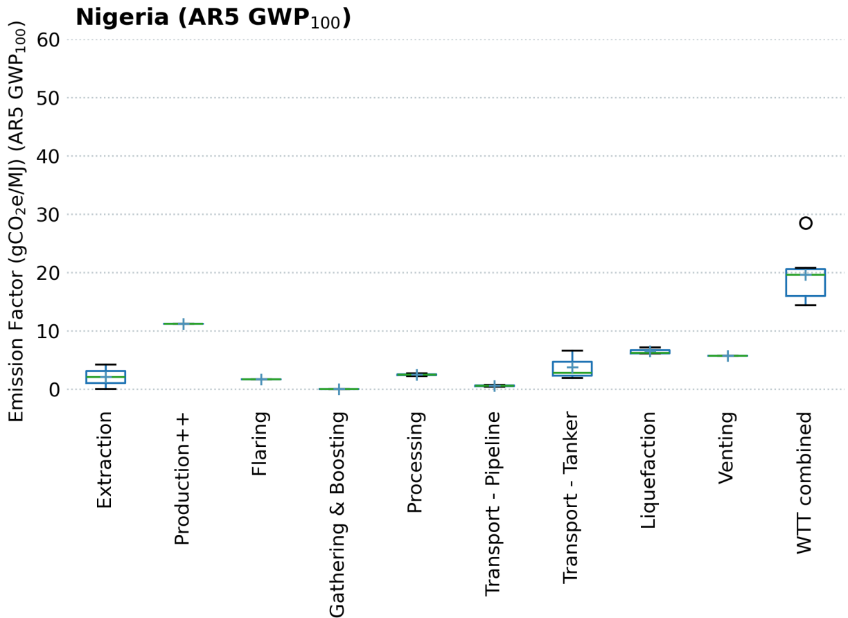
Emission Factors Across LNG Supply Chain in Nigeria (AR5, GWP 100 , gCO 2 e/MJ)
