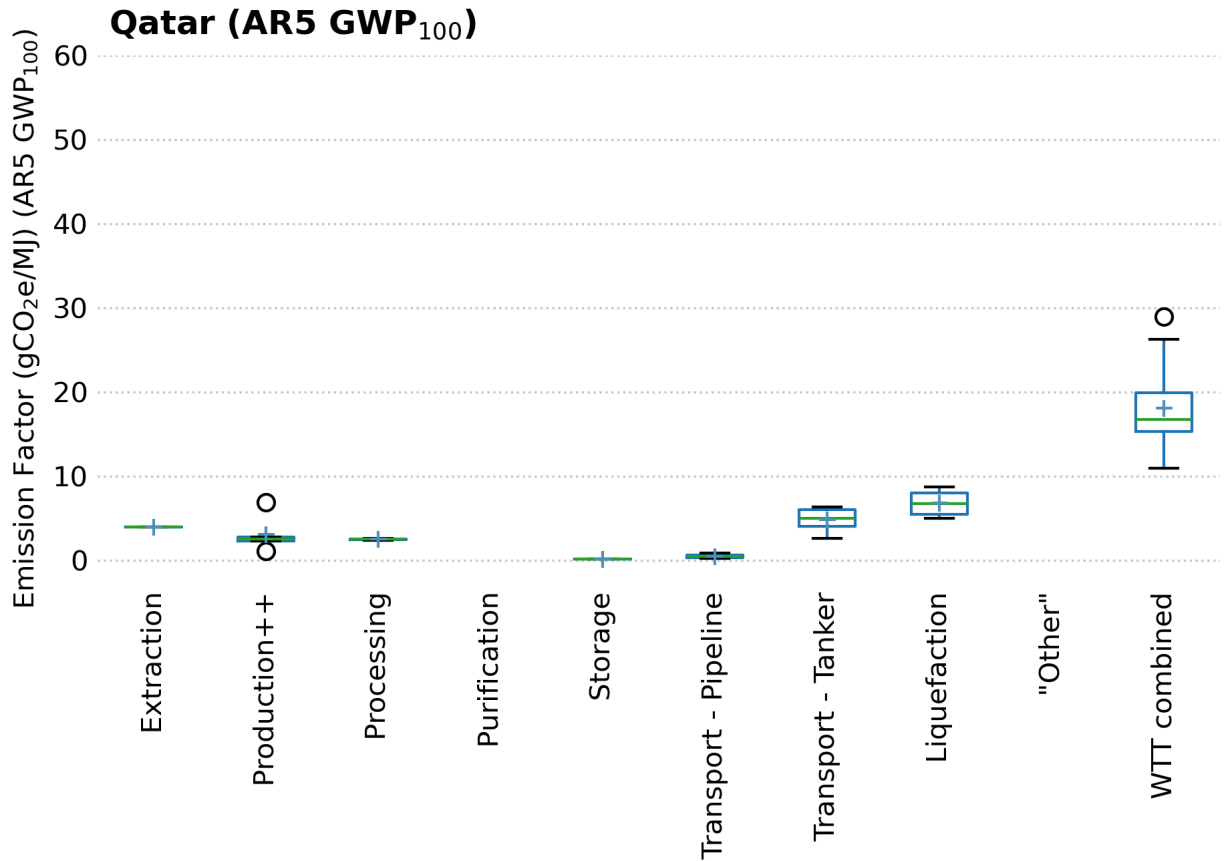
Emission Factors Across LNG Supply Chain in Qatar (AR5, GWP 100 , gCO 2 e/MJ)
