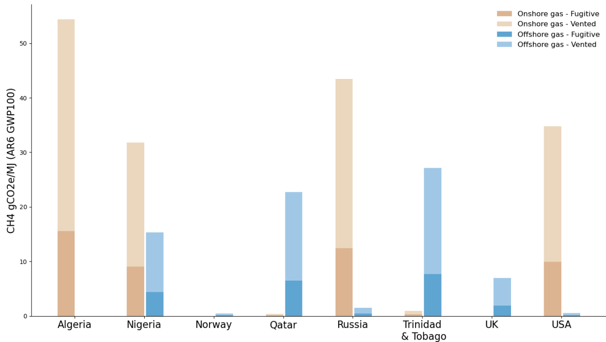
IEA Methane Tracker, Onshore and Offshore Emissions from Upstream Production (AR6, GWP 100 , gCO 2 e/MJ)
