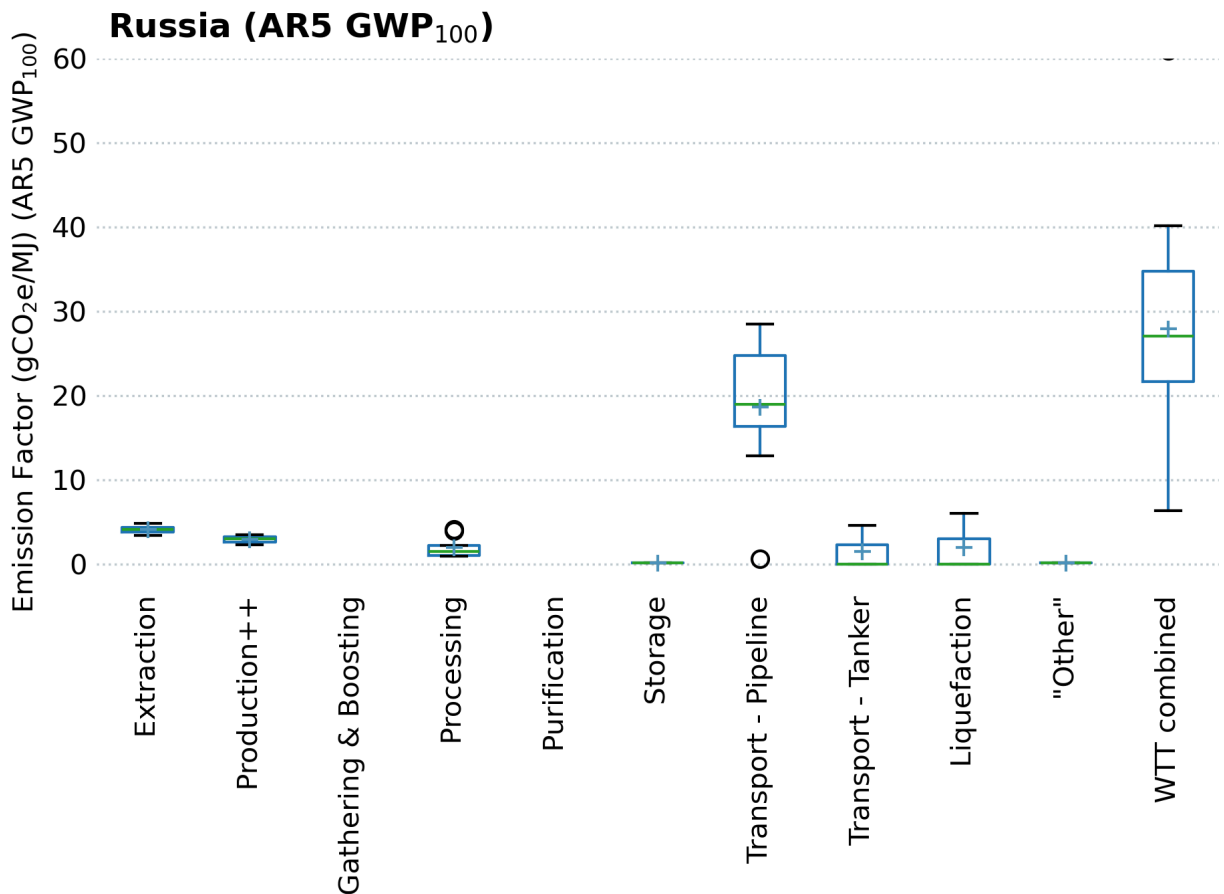
Emission Factors Across LNG Supply Chain in Russia (AR5, GWP 100 , gCO 2 e/MJ)
