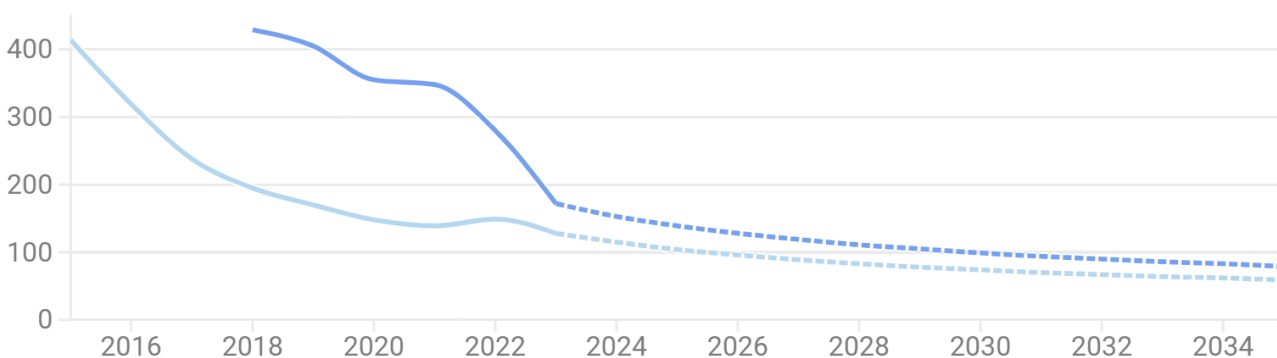
Battery cell and pack prices (real 2023 €/kWh)
